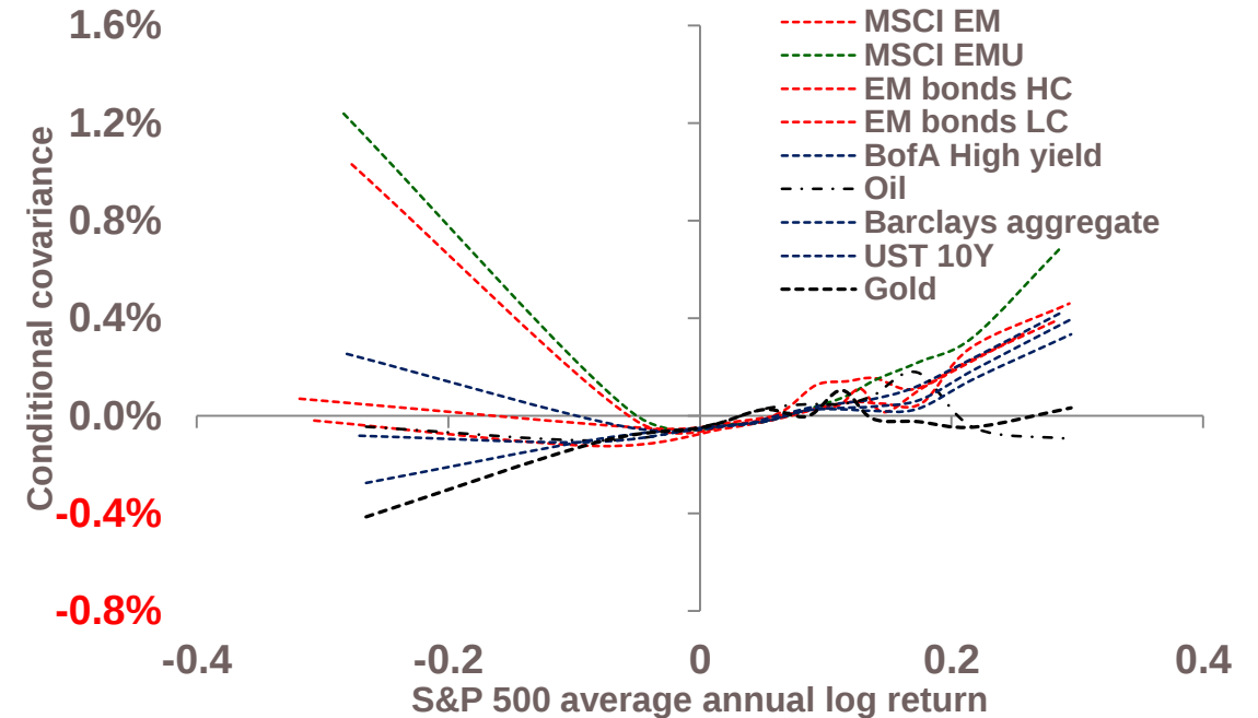
Covariance mapping
